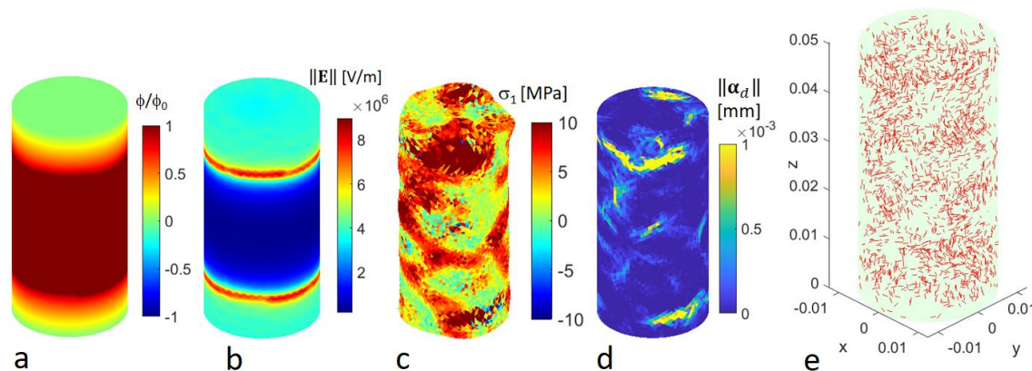
Figure 3. Normalized potential field (a) and the magnitude of electric field at the crest 1 st of cycle (b); Major principal stress field (in the 1000× deformed mesh) (c), crack opening magnitude (d), and crack normal orientations (with every 50th plotted) (e) at the end of simulation.
