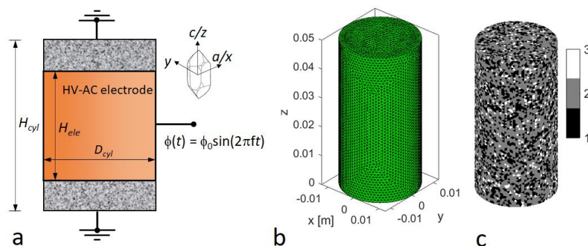
Figure 2. Boundary conditions ( H_{cyl} = 50 mm, H_{ele} = 30 mm, D_{cyl} = 25 mm, \varphi_0 = 50 kV, f = 305 kHz) (a), the finite element mesh with 206617 elements (b), numerical rock mineral texture (3 = Quartz, 2 = Feldspar, 1 = Biotite) (c).
