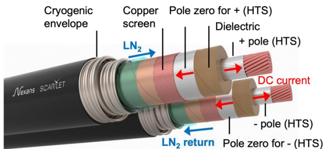
Fig. 4. MVDC power link at 2 GW comprising two HTS cables with two asymmetric concentric poles 0/+100 kV and 0/- 100 kV, with return current in the poles zero and LN 2 circulation in one pole and return in the other.
