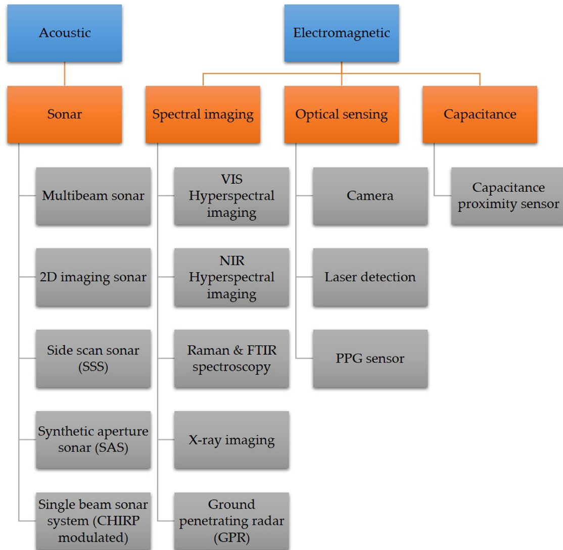
Fig. 2. Conceptual overview of the different technologies that are suitable or have potential to detect plastic on the seafloor.
