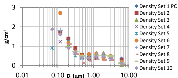
Figure 2: Density correction factors calculated from gravimetrically determined mass-distribution by comparing with measured ELPI- number concentrations.
