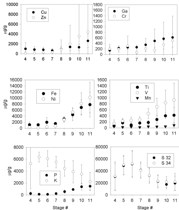
Figure 12: Impurity element distributions in raw-gas particulates.
