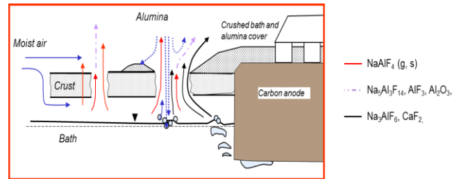
Figure 15: Sketch of particle evolution and entrainment into raw-gases. Quenching and hydrolysis of bath vapours.
