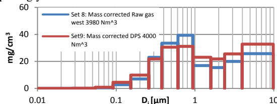
Figure 4: Particle size distribution changes due to DPS-suction. Conventional suction system: 184 \text{ mg}/\text{cm}^3 , Median 1.02 \mu\text{m} . DPS: 202 \text{ mg}/\text{cm}^3 , Median 1.12 \mu\text{m} .
