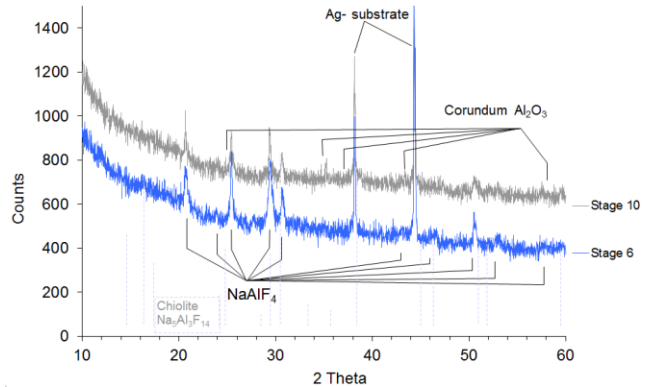
Figure 11: XRD analysis of size classified particles samples Stage 10 D_i=1.95 \mu\text{m} . Stage 6 D_i=0.31 \mu\text{m} .
