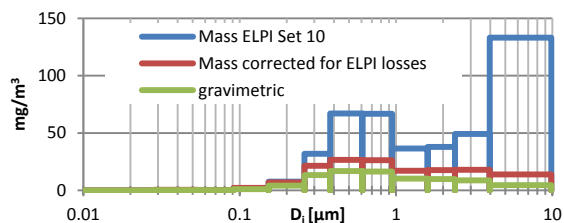
Figure 1: Comparison of mass-concentrations Set 10: Gravimetric (green), corrected for charger losses (red), and as computed by ELPI software based on the assumption of uniform particle density for all particle size classes (blue).
