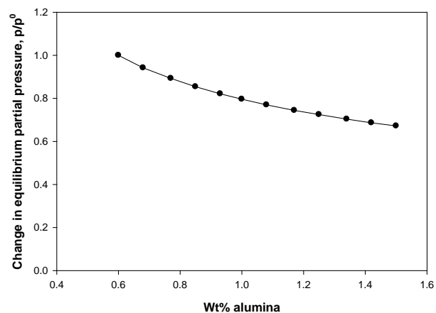
Figure 4: Theoretical change in equilibrium partial pressure for HF as a function of alumina content calculated from Equation 3 at 1000°C. The activity of \text{AlF}_3 and \text{Al}_2\text{O}_3 for each alumina concentration was calculated from Solheim and Sterten [7] .
