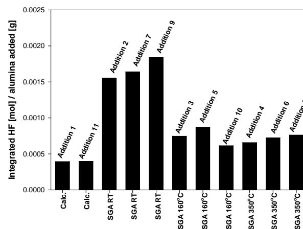
Figure 7: Bar chart showing the impact of the various heat treatments on the SGA on the integrated HF formation.
