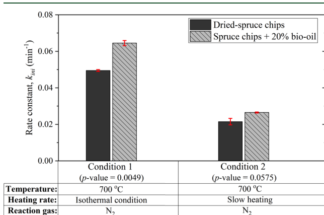
Figure 14. Rate constant in the comparison between the charcoals from bio-oil-embedded woodchips and dried woodchips. The error bars are the standard deviation obtained from two repetitions.
