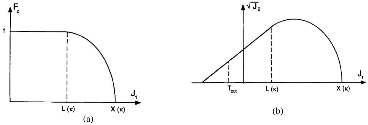
Figure 5. (a) Non-dimensional function used for cap portion of the smooth cap model function. (b) Single smooth cap failure function (from Schwer and Murray, 1994)
