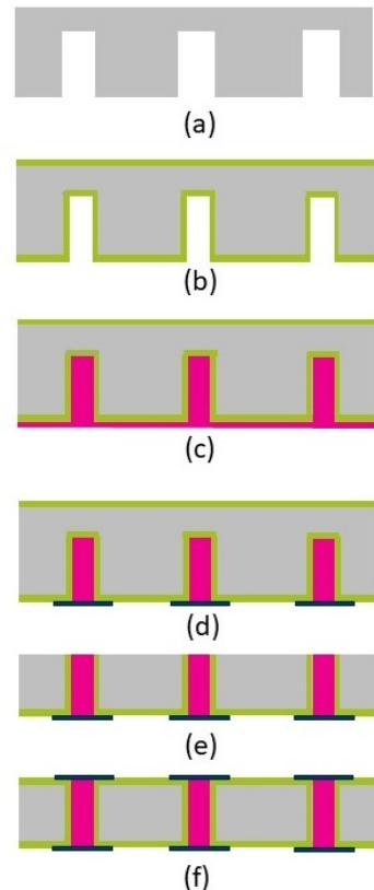
Fig. 3. Possible fabrication of a blind TSV, high aspect ratio silicon etching (a), the vias are then passivated (b) and filled (c). The vias are then electrically connected with a metal layer (d). The wafer is then thinned to reveal the vias by a CMP process (e). The vias are then completed with a second metal layer on the back side of the wafer (f).
