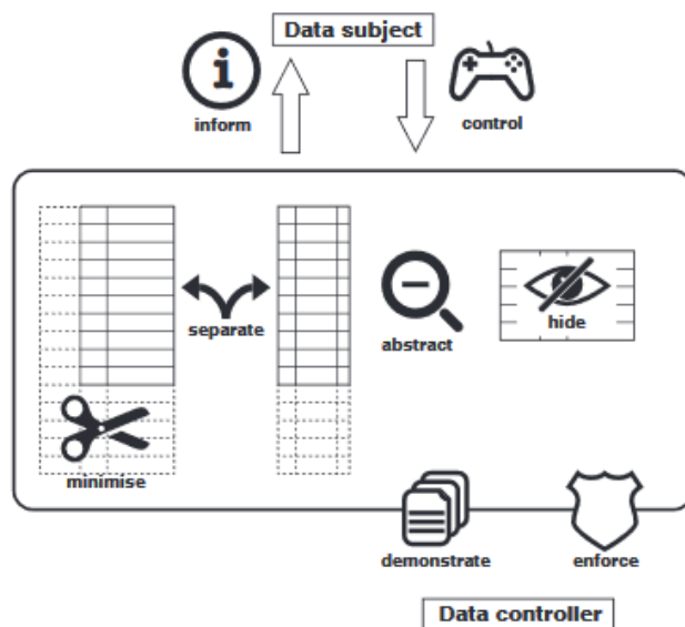
Fig. 1: An illustration of eight privacy design strategies for a database [Hoepman, 2018]. The strategies can be transferred to event logs and, thus, serve as requirements for the design of privacy-preserving process mining systems.
