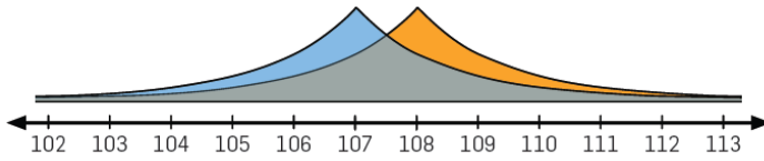
Fig. 4: Adding random noise to the result of a counting query using the Laplace distribution as illustrated in [McSherry, 2010]. This transformation ensures differential privacy while keeping the noisy result close to the original value.
