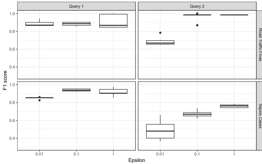
Fig. 6: F1 score based on the projected recall and precision measures when comparing the process model discovered on the unprotected data without our protection method and on the privacy-protected event log for both processes. Each box plot is based on 10 repetitions.
