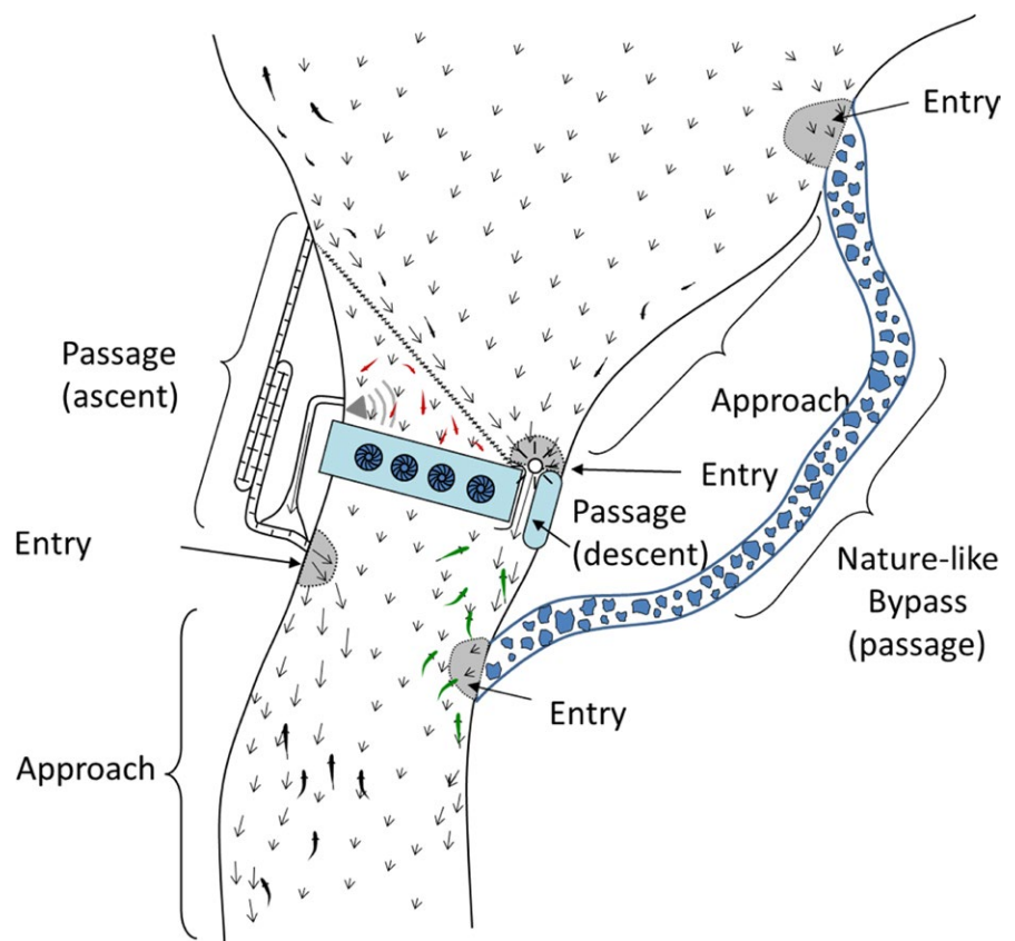
FIGURE 1 Phases of fish passage applied to any obstacle with fishway(s), herein illustrated for a powerhouse equipped with separate up- and downstream fishways (adaptation of Castro-Santos & Haro, 2010) [Colour figure can be viewed at wileyonlinelibrary.com ]
