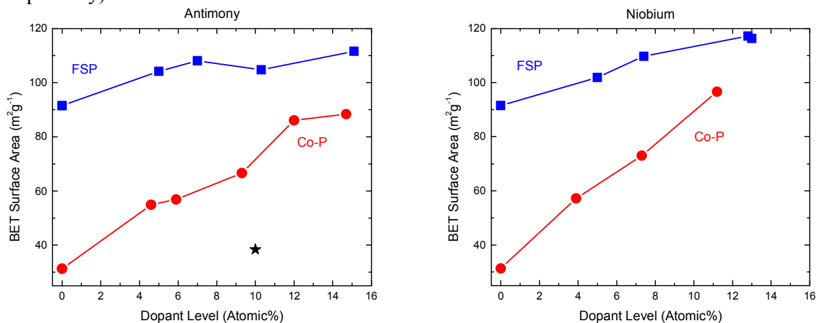
Figure 1. Surface area of as synthesized tin oxide powders prepared by FSP and Co-P as a function of Sb and Nb doping. Star in graph to the left indicate data from commercial material.
