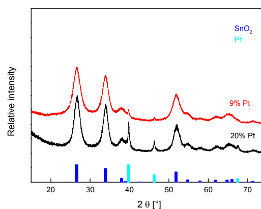
Figure 4. XRD analysis of Pt supported on \text{Sn}_{0.935}\text{Sb}_{0.065}\text{O}_{2+\delta} by one-step FSP route.
