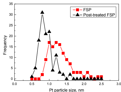
Figure 6. Pt particle size distribution from TEM analysis for the samples depicted in Figure 5 c) and d).
