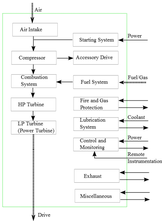
Fig. 1. Sub-systems of an industrial gas turbine engine
