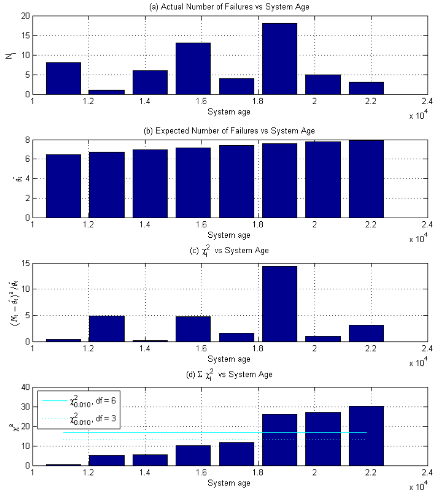
Fig. 13 : Chi-square statistics
