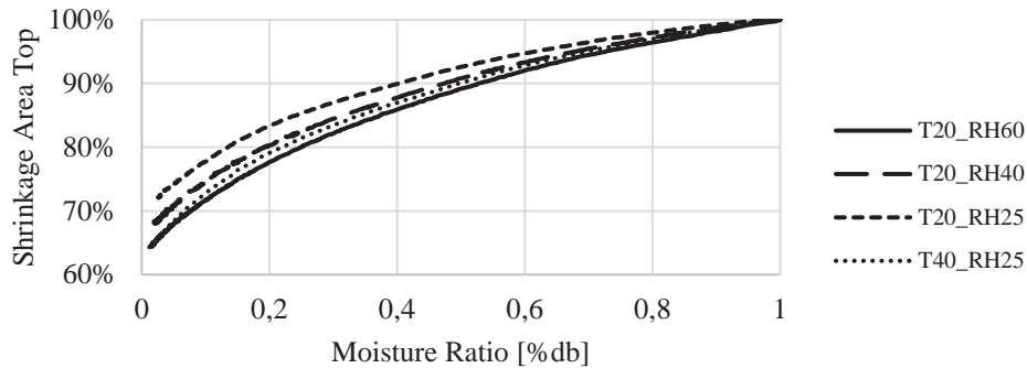
Figure 5: Top view shrinkage of organic apples at different drying conditions.
