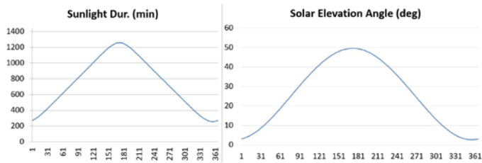
Figure 2 Sunlight duration (left) and solar elevation angle (right) at all days of 2016, as seen from the location of the PV panel 1
