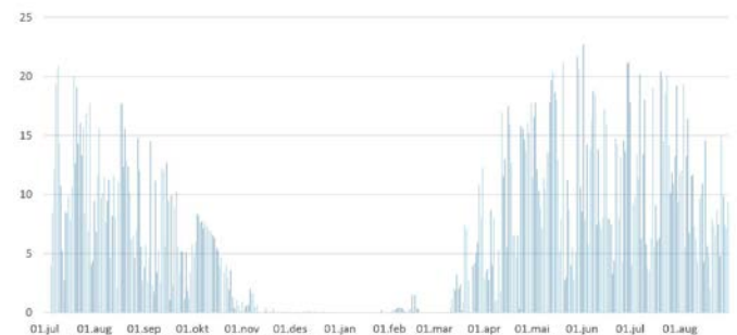
Figure 1 Daily PV production 2016.07.05 – 2017.08.31 [kWh]
