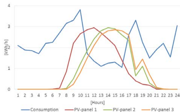
Figure 4 Changes in feed-in of electricity, as a consequence of the orientation of the PV-panel
