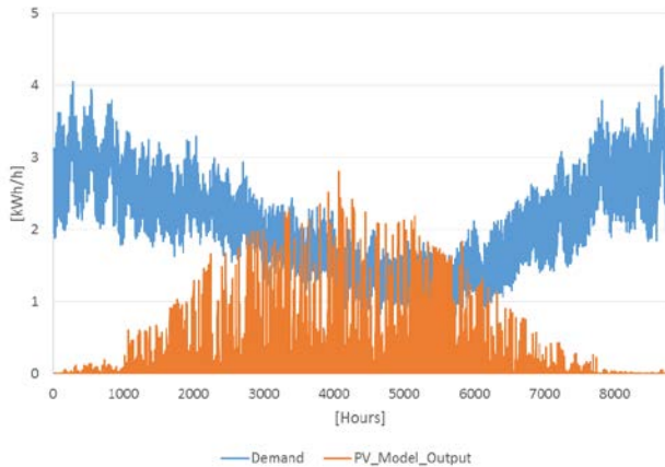
Figure 2 Load curve for typical residential customer and modelled PV-generation
