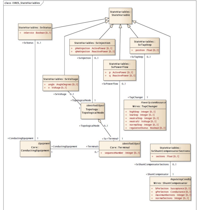
Fig. 10. State Variable profile
