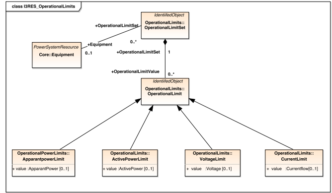
Fig. 7. Operational limits of typical equipment class
