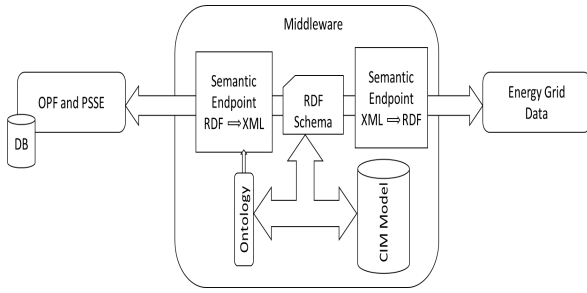
Fig. 13. CIM Integration with the Middleware Using Ontology
