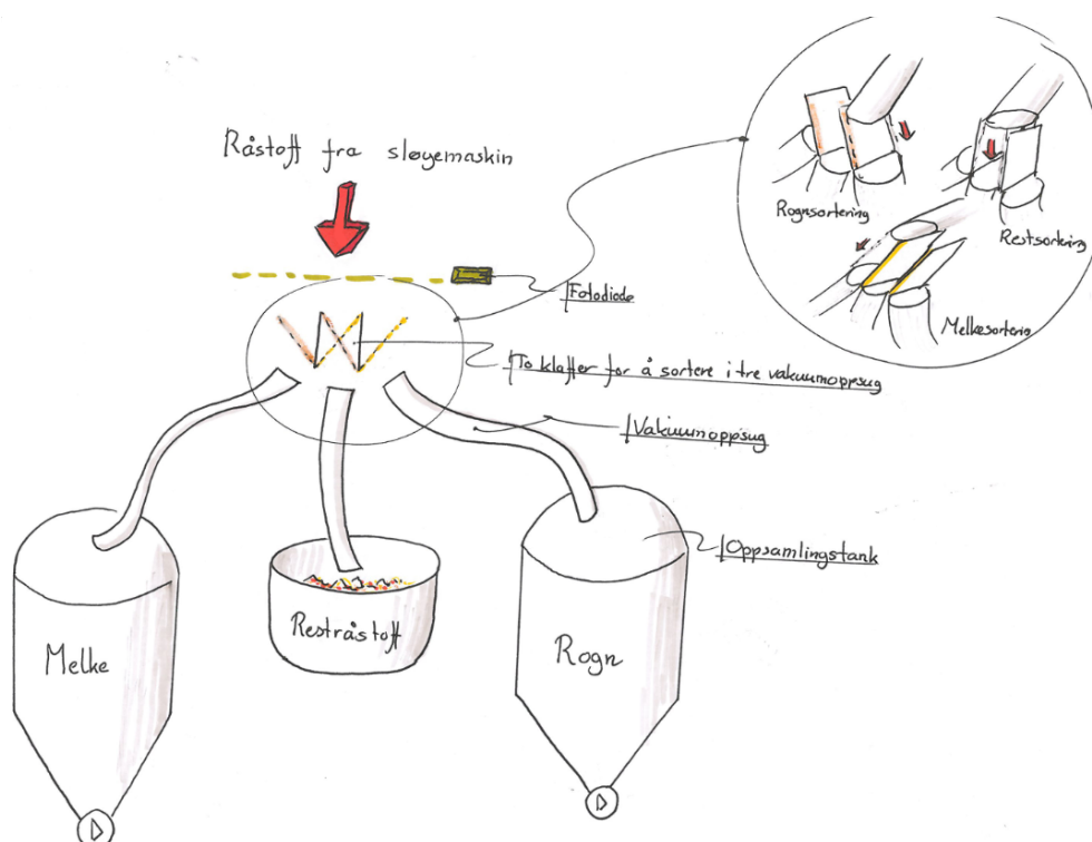
Figur 4-6: Konseptskisse "QuickSort"
