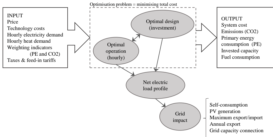
185 Figure 2 Model description with main inputs and outputs. Grid impacts are consequences of the optimal design and operation.
