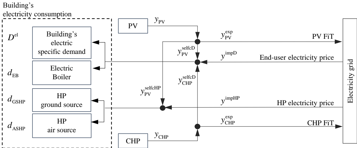
Figure 3 Detailed graphical explanation of the electricity flows in Figure 1, together with their electricity price or export value.
