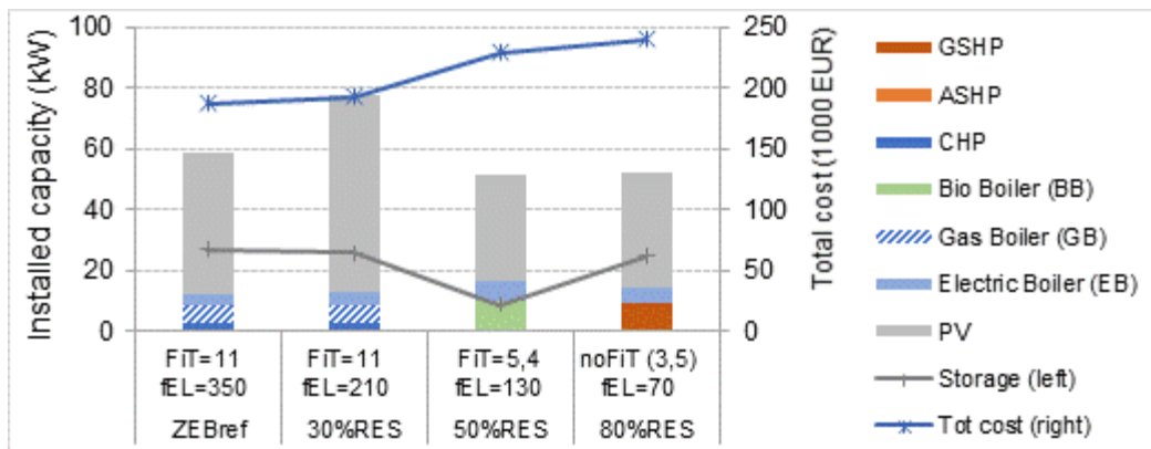
Figure 13 Results of greener electricity production mix. Influence of reduced weighting factors for electricity ( f_{EL} ), combined with lower FiT for PV (ct/kWh), on installed capacity (kW) and total discounted cost (1000 EUR).
