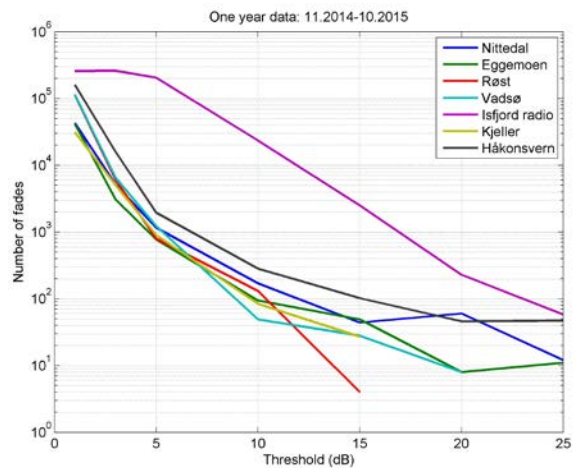
Fig. 6. Measured number of fades.
