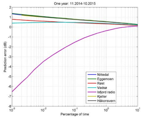
Fig. 5. Prediction error of scintillation and multipath.
