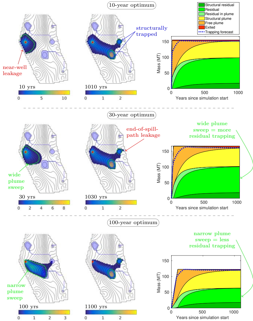
Fig. 5: Optimal solution given a 10-year, 30-year, and 100-year injection period, for a single-well scenario in Sleipner. Left to right: CO 2 saturations at end of injection period and after 1000 years of post-injection, and trapping inventories. Well location is indicated by red dot, and is identical in all three cases. Colorbars refer to tonnes of CO 2 per lateral square meter.
