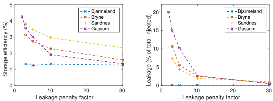
Fig. 7: Impact of leakage penalty factor on the optimized storage efficiency (left) and amount of leakage (right) of select formations.
