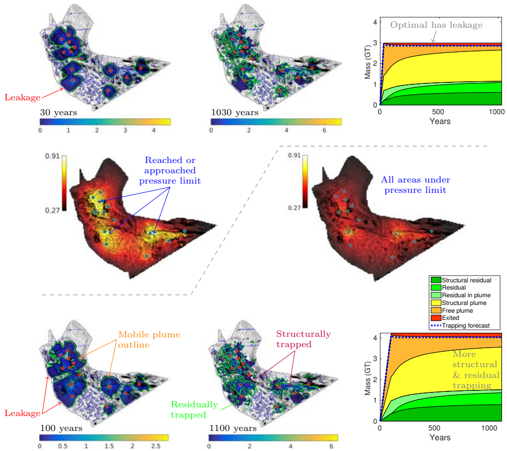
Fig. 6: Comparison of the optimal solutions given a 30-year (top portion) and 100-year (bottom portion) injection period in Sandnes. Top left to top right: CO 2 saturations at end of injection and end of simulated period, and trapping inventory. Middle: fraction of overburden pressure reached. Saturation colorbars refer to tonnes of CO 2 per lateral meter squared. Predefined pressure limit is 0.9 times overburden pressure.
