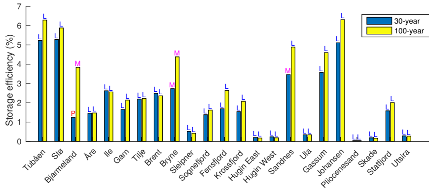
Fig. 3: Categorization of open system formations in terms of what limited their storage efficiency ( S_{\text{eff}} ), given two different injection time frames. S_{\text{eff}} was determined dynamically by optimizing the well injection rates and then by (1). “P” stands for pressure-limited, “L” stands for leakage-limited, and “M” stands for mixed (i.e., limitation due to a combination of pressure and leakage). Results are not intended for engineering purposes.
