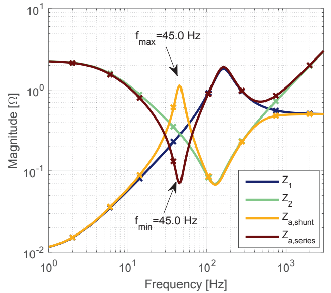
Fig. 7: Impedance curves obtained from intersection A . 'x' represents the simulated values at f_{inj} (14), while the solid lines represent interpolation by Vector Fitting
