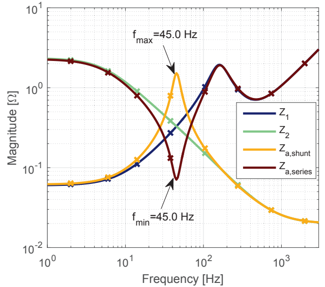
Fig. 8: Impedance curves obtained from intersection B . 'x' represents the simulated values at f_{inj} (14), while the solid lines represent interpolation by Vector Fitting
