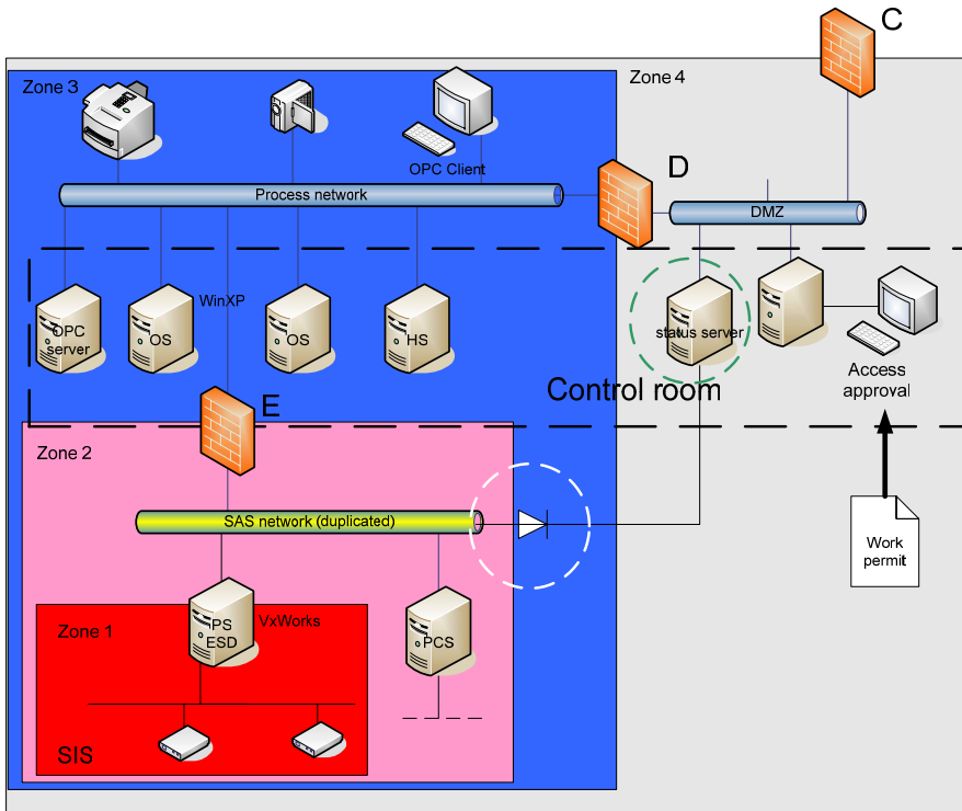
Figure 5 Introduction of information diode for read-only access
