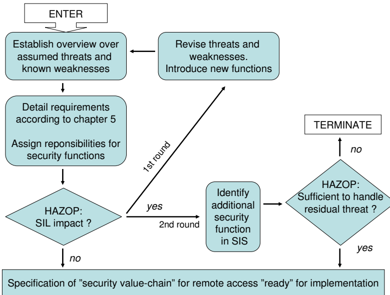
Figure 6 The SeSa method
