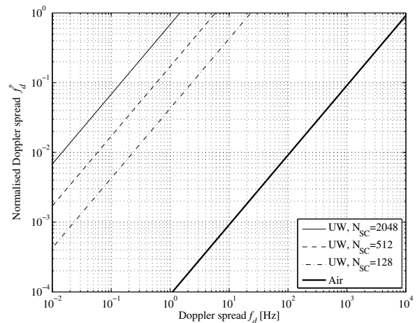
Figure 11 f_d^* for underwater communication
