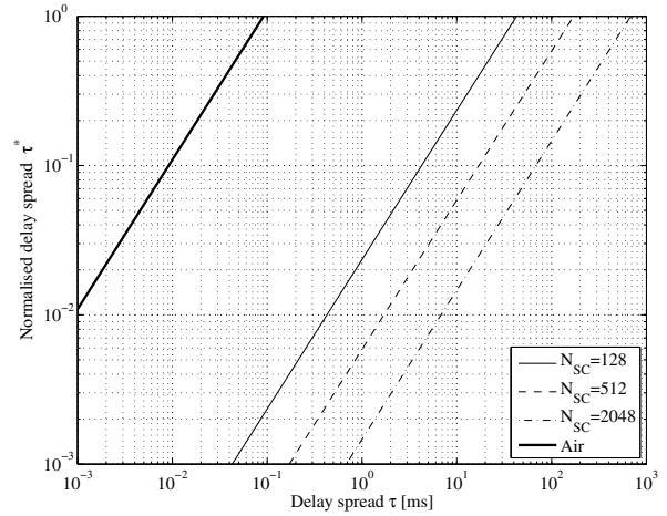
Figure 12 \tau^* for underwater communication
