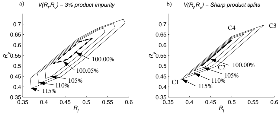
Figure 5: The whole solution surface V(R_p, R_v) is widened for non-sharp products. The plots show contours of the solution surfaces for 3% product impurity (a) and for sharp product splits (b) ( V=100\% in the optimality region). Note the characteristic sharp corners denoted C1-C4 on the sharp-split contours.
