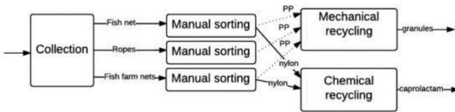
Figure 6 Diagram illustrating how fish nets, fish farming nets and rope can be recycled, based on process at Nofir/Aquafil (Brodbeck, 2016).
