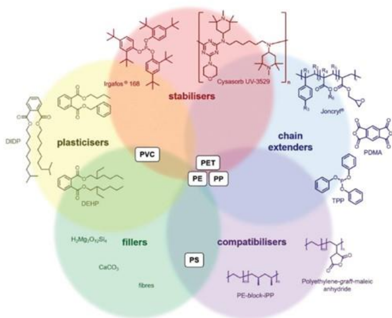
Figure 6 Common polymer additives used to improve polymer recyclates (Schyns and Shaver, 2021)
