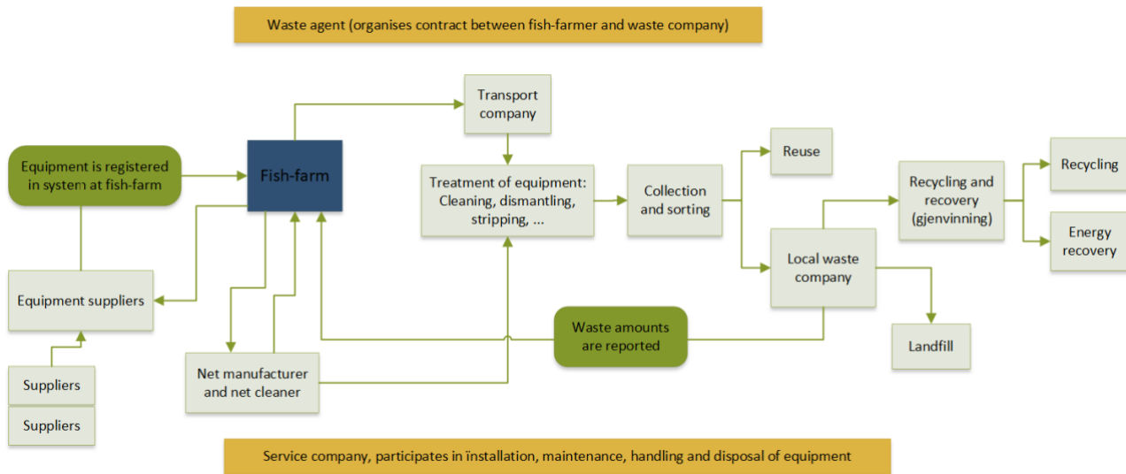
Figure 5 Actors, mass and information flow in the material flows in an aquaculture facility (Hognes and Skaar, 2017)
