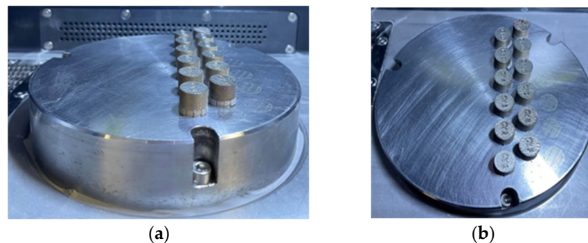
Figure 1. Images of (a) DSS (2205) and (b) SDSS (2507) samples for parameter optimization, prior to removal from the substrate.
