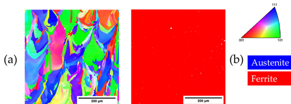
Figure 10. EBSD results of the XZ plane in the as-built DSS sample. (a) Inverse pole figure map: \langle 001 \rangle directions shown in red; \langle 101 \rangle directions in green; \langle 111 \rangle directions in blue. (b) Phase map.
