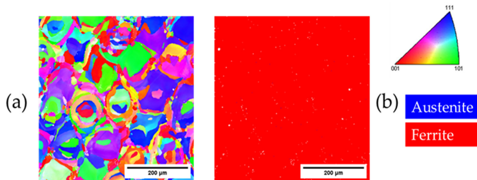
Figure 9. EBSD results of the XY plane in the as-built DSS sample. (a) Inverse pole figure map: \langle 001 \rangle directions shown in red; \langle 101 \rangle directions in green; \langle 111 \rangle directions in blue. (b) Phase map.
