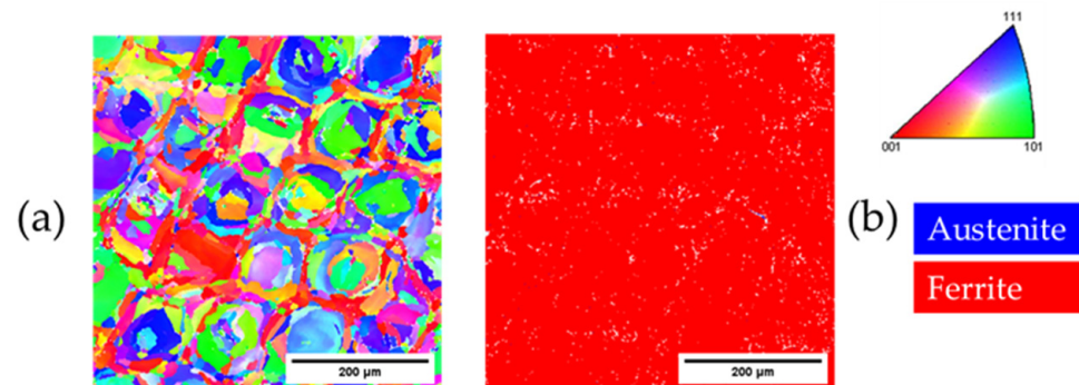
Figure 17. EBSD results of the XY plane in the as-built SDSS sample. (a) Inverse pole figure map: \langle 001 \rangle directions shown in red; \langle 101 \rangle directions in green; \langle 111 \rangle directions in blue. (b) Phase map.
