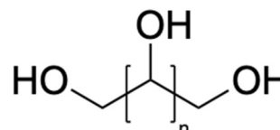
Fig. 3. Sugar alcohol.
