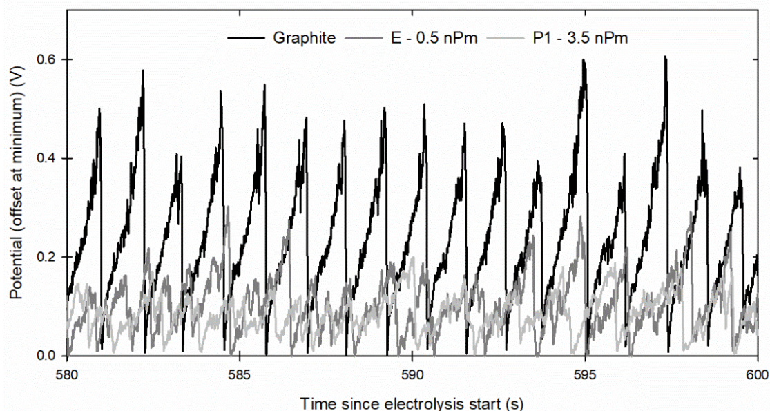
Fig. 4 – Examples of the measured potential vs time for graphite, the anode with lowest permeability and highest permeability. The graphs have been shifted to a similar offset (0).
