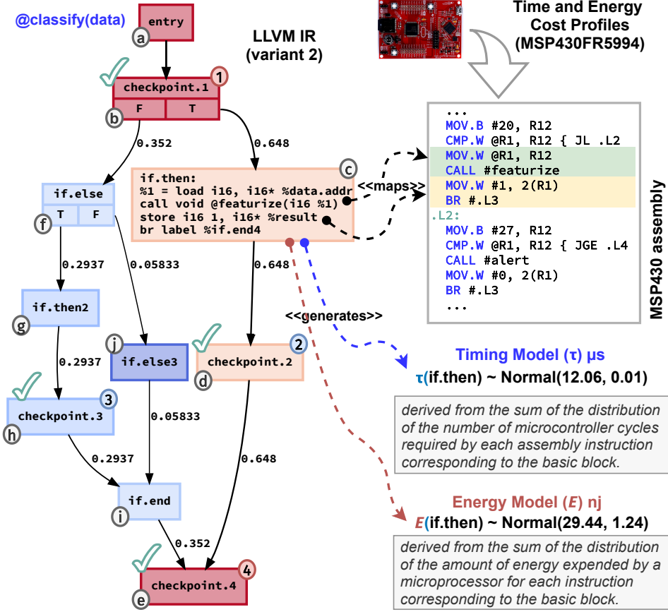
Fig. 5. Control Flow Graph of Function classify with Program Variant #2. The figure shows the timing ( \tau ) and energy ( E ) cost models of basic block if.then , which are automatically derived from the mapping between the basic block in LLVM IR and the compiled target MSP430 assembly. Basic block if.then calls featurize() ; basic block if.then2 calls function alert() ; and basic block if.else3 calls function error() . ETAP generates a basic block for each call to checkpoint() function.
