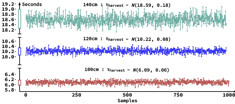
Fig. 8. RF energy profiles: charging-time samples for a 50mF supercapacitor at different distances.
