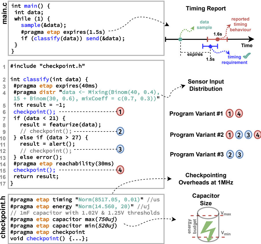
Fig. 4. Example Intermittent Program with ETAP Pragmas. In the classify function, featurize and alert function calls are expected to take relatively more time and consume more energy. Therefore, to save the progress of computation, the programmer may apply alternative checkpoint configurations such as adding checkpoints before and after every major computation conservatively (Program Variant #2 has checkpoints 1, 2, 3, and 4); or placing checkpoints at enter and exit of the function (Variant #1 has only checkpoint 1 and 4—checkpoints colored with red in the figure); or saving the progress of featurize or alert computations separately (Variant #3 has checkpoint 2 and 3—checkpoints colored with blue in the figure). The question that ETAP can answer is which checkpoint placement strategy would meet the given timing requirement best under a set of given capacitor alternatives.
