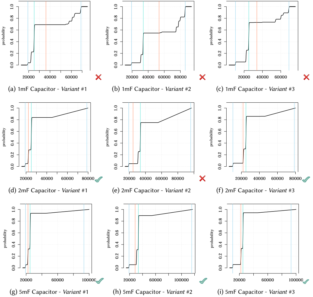
Fig. 7. Reports of the Execution Time Probability Distributions (Cumulative Distribution Function) of Function classify after symbolically executing with 1MHz clock-rate under 3 different capacitor type and 3 different checkpoint placements with the given \tau_{\text{harvest}} profiles. The values on x-axis are in microseconds. The blue vertical lines represent the first quartile , the median , and the third quartile respectively; the red vertical line is the mean of the probability distributions.
