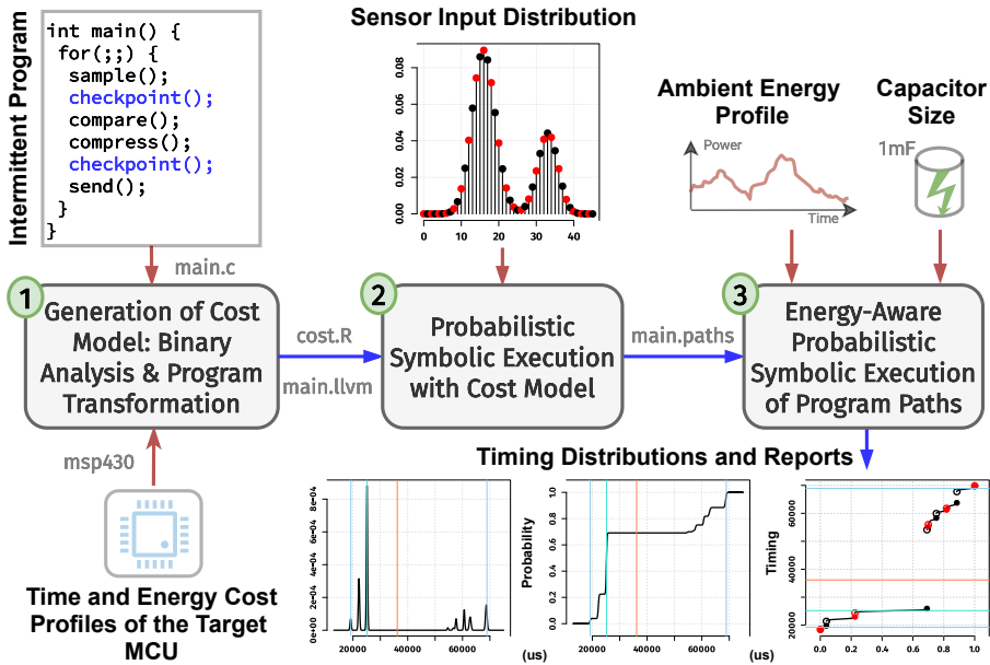
Fig. 3. ETAP consists of three stages after inputs are specified (see Section 5): (i) Generation of cost models using binary analysis and program transformation (see Section 6), (ii) Probabilistic Path Exploration that generates probabilities of execution traces based on sensor input distributions and program semantics (see Section 7), and (iii) Energy-aware symbolic execution based on intermittent execution of program semantics, microcontroller’s energy consumption, and capacitor’s energy capacity (see Section 8). Under given configurations, ETAP generates reports about timing distributions.
