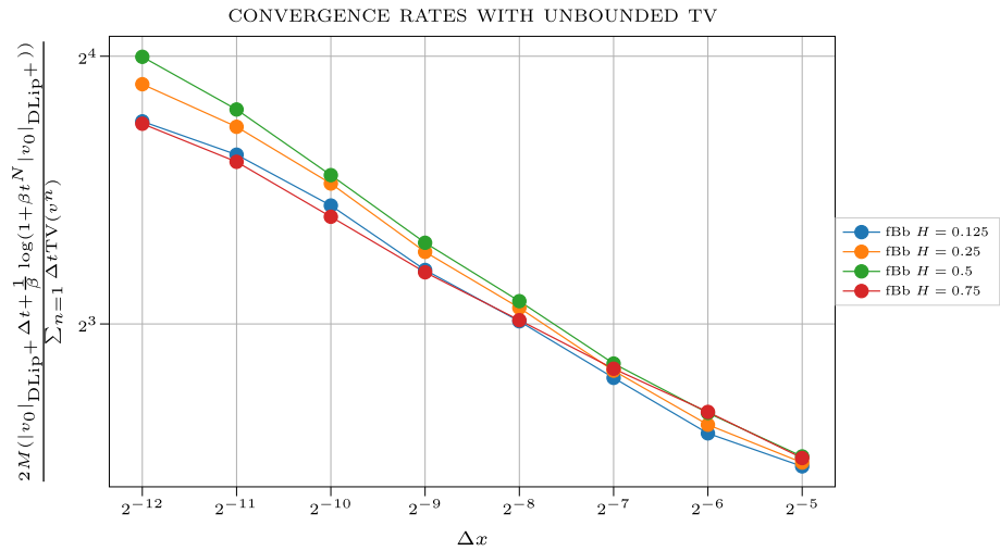
Fig. 6 Sharpness of the bound (12) for Burgers’ equation solved with the Godunov scheme. Specifically, we plot the ratio \frac{2M(|v^0|_{DLip} + \Delta t + \frac{1}{\beta} \log(1 + \beta t^N |v^0|_{DLip}))}{\sum_{n=0}^N TV(v^n) \Delta t} as a function of the mesh width \Delta x . A value of 1 corresponds to a sharp estimate, a value greater than one corresponds to an not sharp estimate
