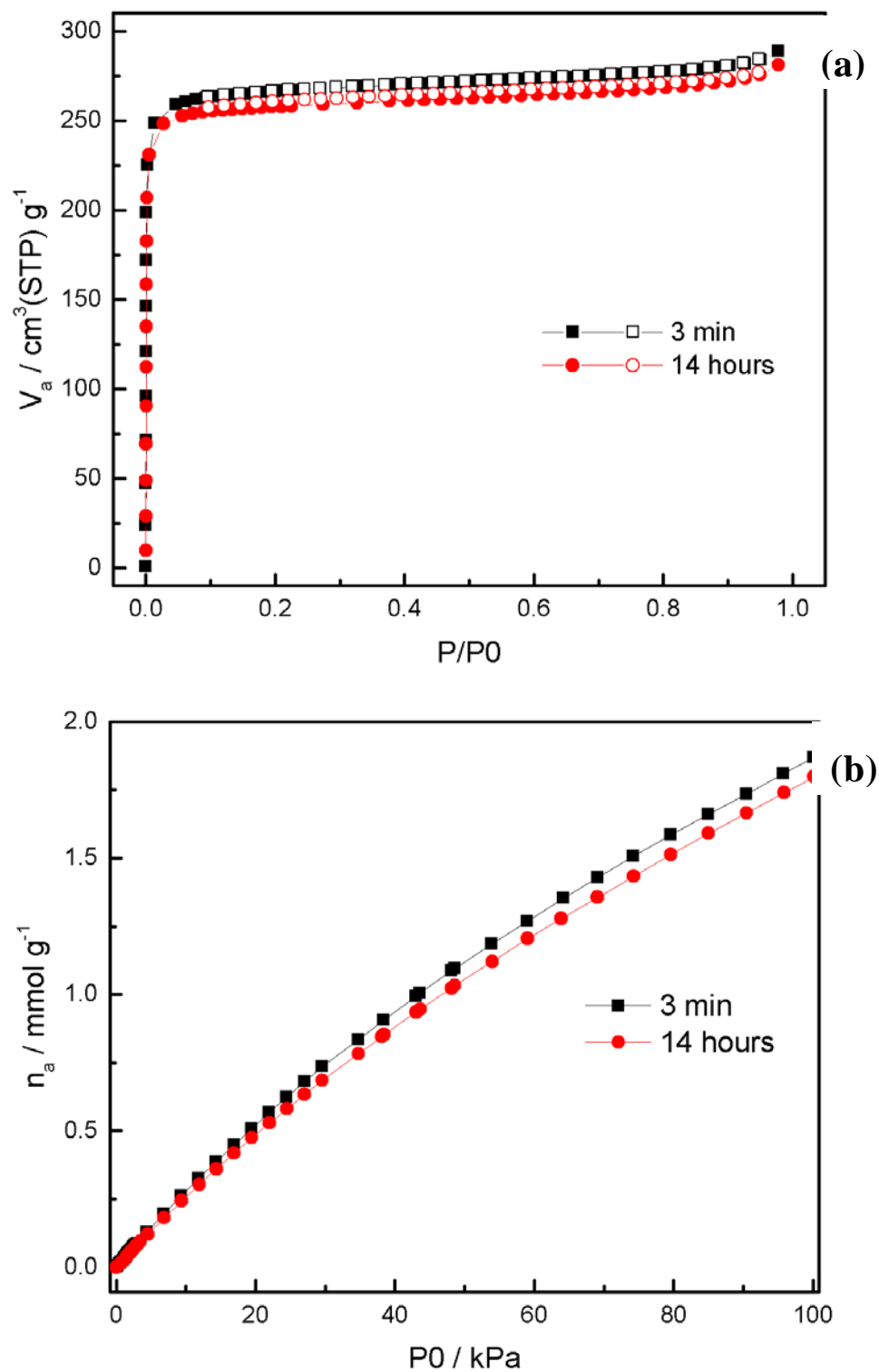
Figure 8: Nitrogen sorption isotherm at 77K (a) and \text{CO}_2 isotherms at 298 K (b) on DWL-11.
