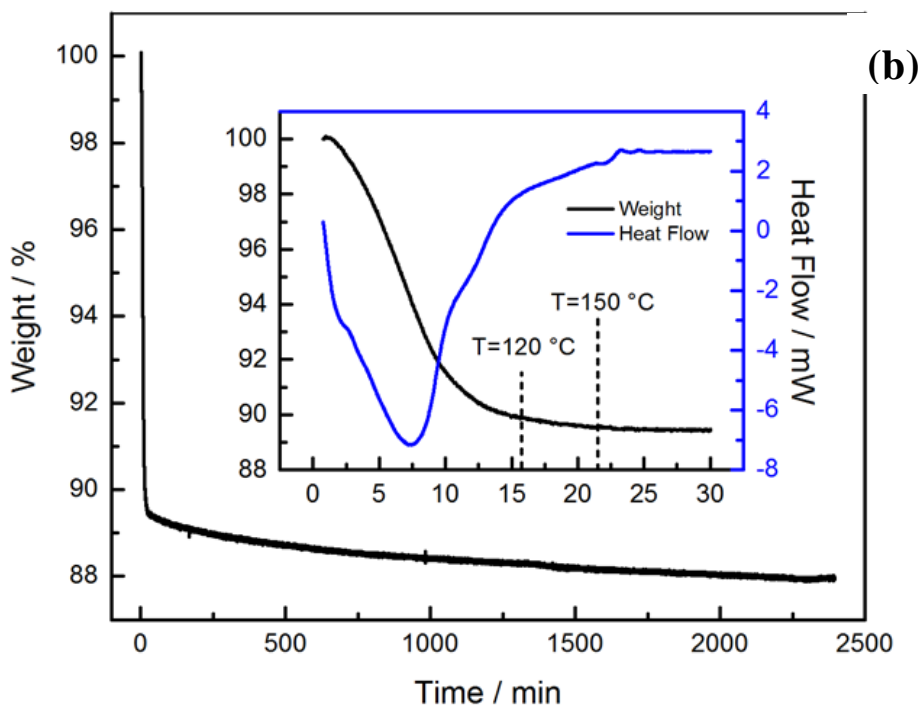
Figure 13: TGA data of DWL-9-1.8% at three different activation temperatures a) TGA data of DWL-9-1.8% at three different activation temperatures; 120, 135 and 150°C. b) More details of TGA activation of DWL-9-1.8% at 150°C showing that stable mass is still not reached after 2500 min. Insert: TGA and DSC details for the first 30 minutes showing the heat flow during the initial phase of the activation
