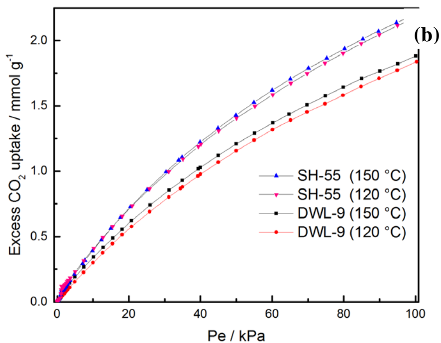
Figure 16: Nitrogen adsorption isotherm at 77K (a) and CO 2 uptake at 298 K (b) on powder (SH-55) and on beads (DWL-9) activated at two different temperatures: 120 °C and 150 °C.
