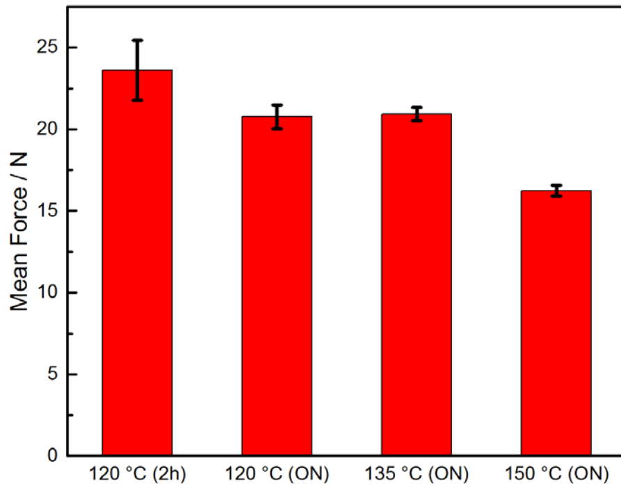
Figure 15: Average crushing strength of DWL-9-1.8% after 4 different activation conditions: activation at 120 °C for 2 hours, 120 °C overnight, 135 °C overnight, 150 °C overnight. Red bars illustrate the mean value and the error bars indicate the difference between the maximum and the minimum value.
