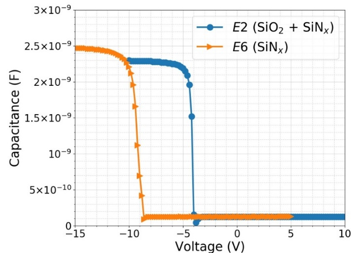
Figure 10. Capacitance—voltage (C—V) measurement results of MIS capacitors prepared with the passivation processes E2 (6 nm \text{SiO}_2 + 65 nm \text{SiN}_x ) and E6 (65 nm \text{SiN}_x ) as described in Table 1, at a frequency of 1 kHz.
