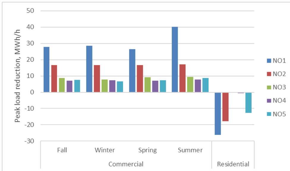
Figure 60. Peak load reduction per region in Petroleum Nation 2050 with use of flexible electric water heater, GWh/h
