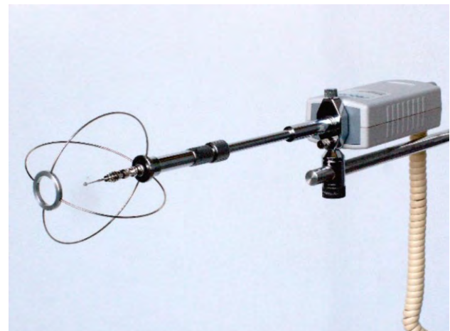
Figure 4. AirDistSys5000
