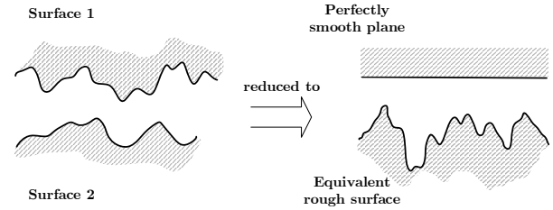
Fig. 2: Contact asperities between a perfectly smooth surface and a rough surface. Greenwood and Tripp [1] showed that the contact of two rough surfaces could be reduced to a so-called equivalent sum surface, consisting of a single, rough surface with a smooth, rigid plane. For details, refer to Chapter 3 in [5].
