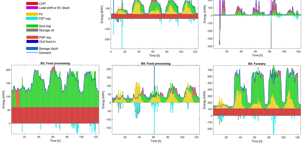
Fig. 3. Supply–demand results for the Shared Storage Case in a summer week.
