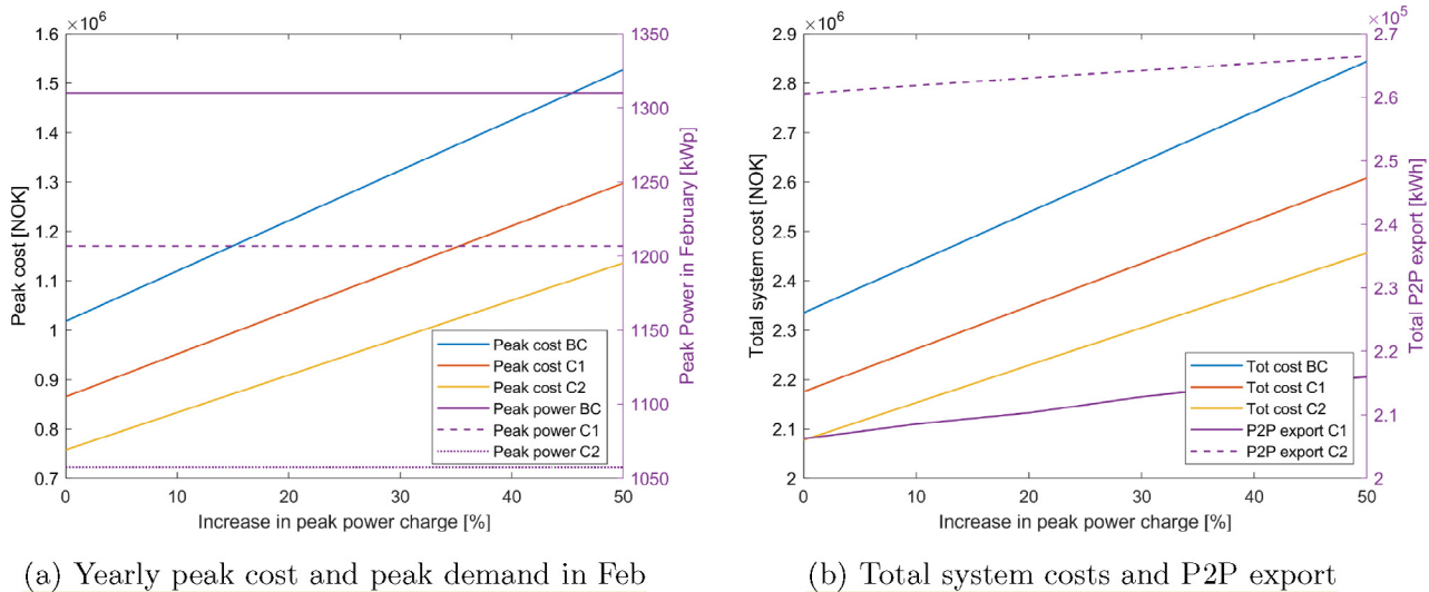
Fig. 4. Sensitivity to percentage change in the peak power demand charge.
