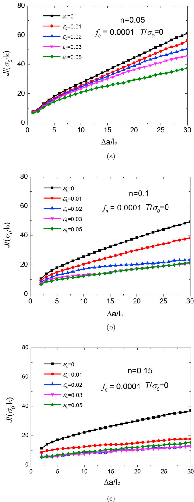
Fig. 9. Effect of Lüders plateau on resistance curves for materials with different strain hardening: (a) n = 0.05 ; (b) n = 0.1 ; (c) n = 0.15 .
