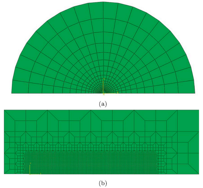
Fig. 2. Modified boundary layer model used for numerical analysis: (a) Global mesh; (b) Local mesh.
