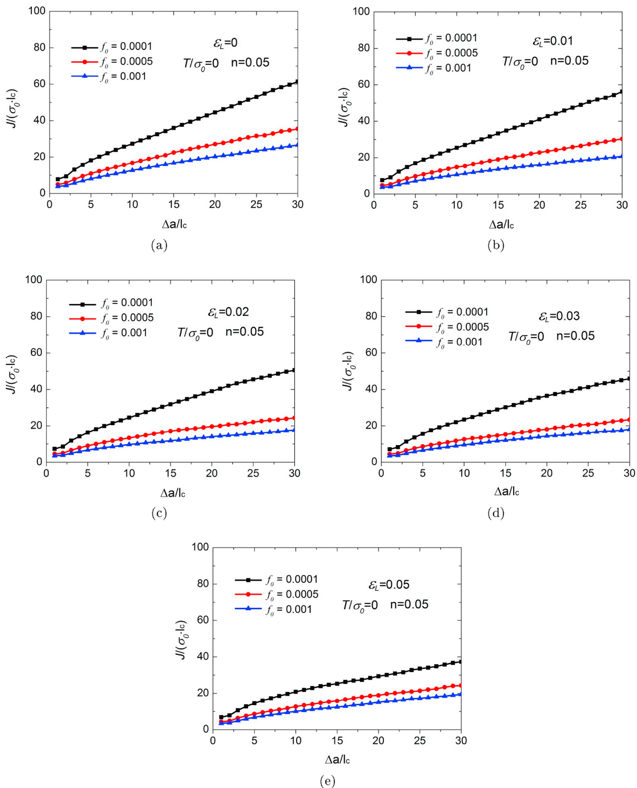
Fig. 11. Resistance curves dependence on the initial void volume fraction for materials with the same Lüders elongation: (a) \epsilon_L = 0 ; (b) \epsilon_L = 0.01 ; (c) \epsilon_L = 0.02 ; (d) \epsilon_L = 0.03 ; (e) \epsilon_L = 0.05 .
