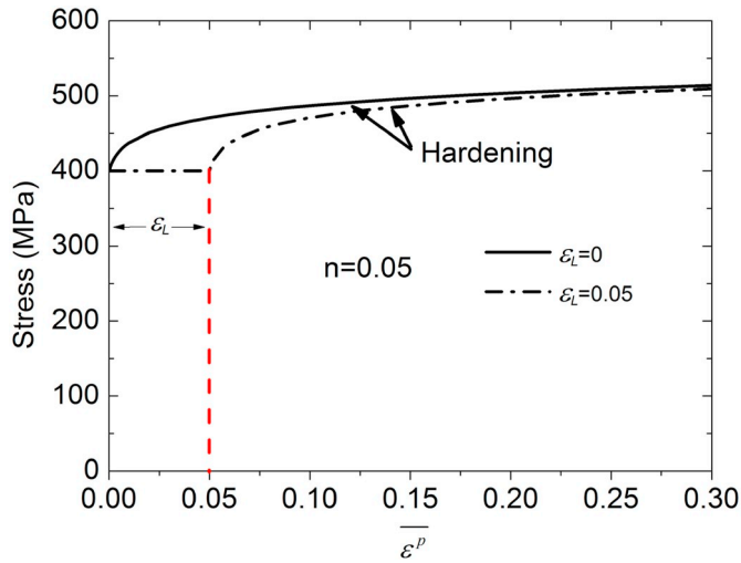
Fig. 1. Illustration of the flow stress-strain curve with Lüders plateau used in this study.
