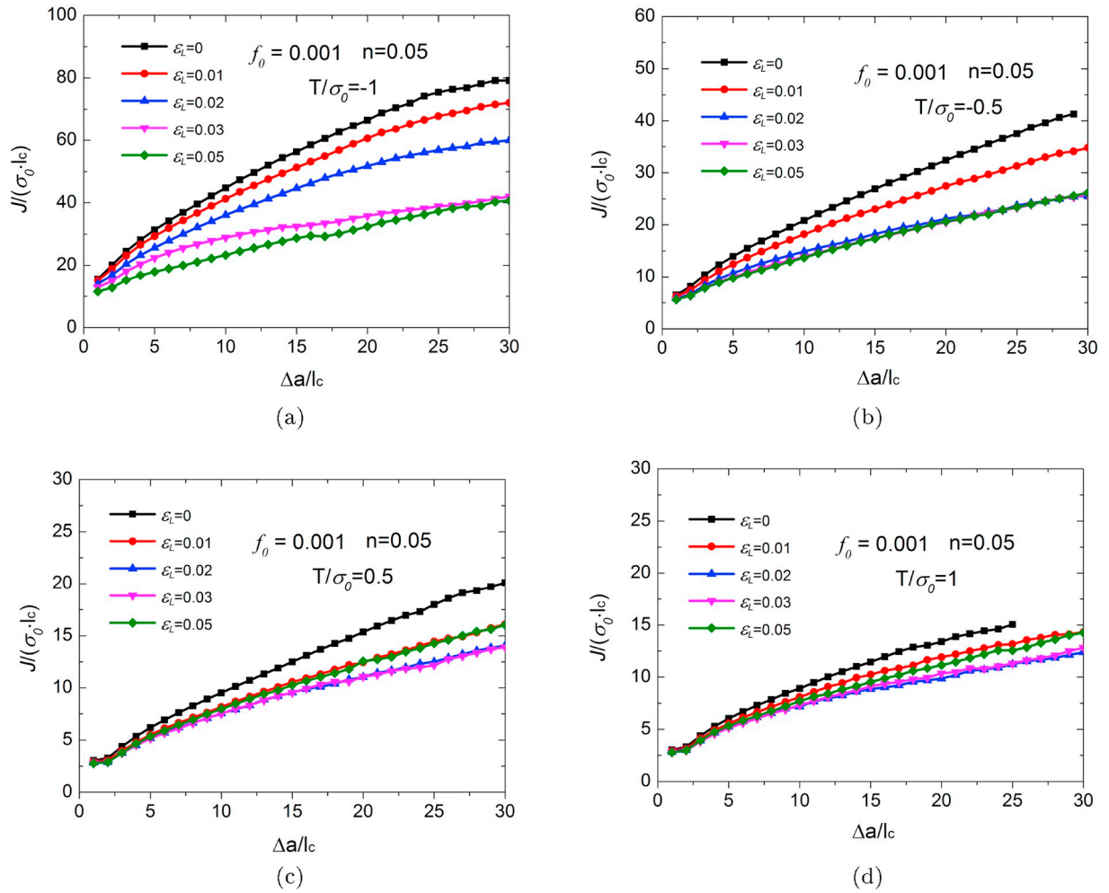
Fig. 7. Resistance curves from MBL model under different T -stresses: (a) T/\sigma_0 = -1 ; (b) T/\sigma_0 = -0.5 ; (c) T/\sigma_0 = 0.5 ; (d) T/\sigma_0 = 1 .
