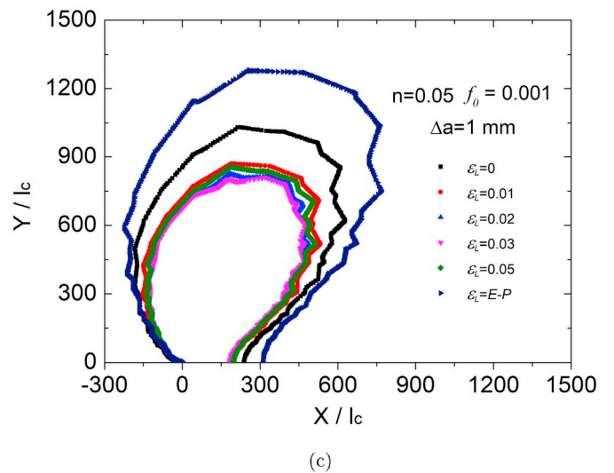
Fig. 6. Plastic zone size at given crack increment: (a) \Delta a = 0.1 mm; (b) \Delta a = 0.5 mm; (c) \Delta a = 1 mm.
