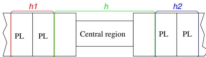
Figure 14: Schematic illustration of the transport setup and the matrices h_1 , h and h_2 defining the left lead, central region and right lead, respectively.
