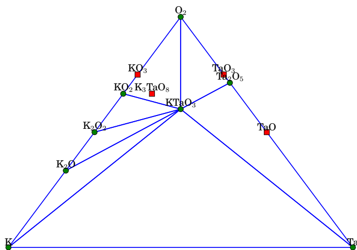
Figure 10: Phase diagram for K-Ta-O. The stable phases are indicated by green circles and are vertices of triangles. The unstable compounds are indicated by red squares.
