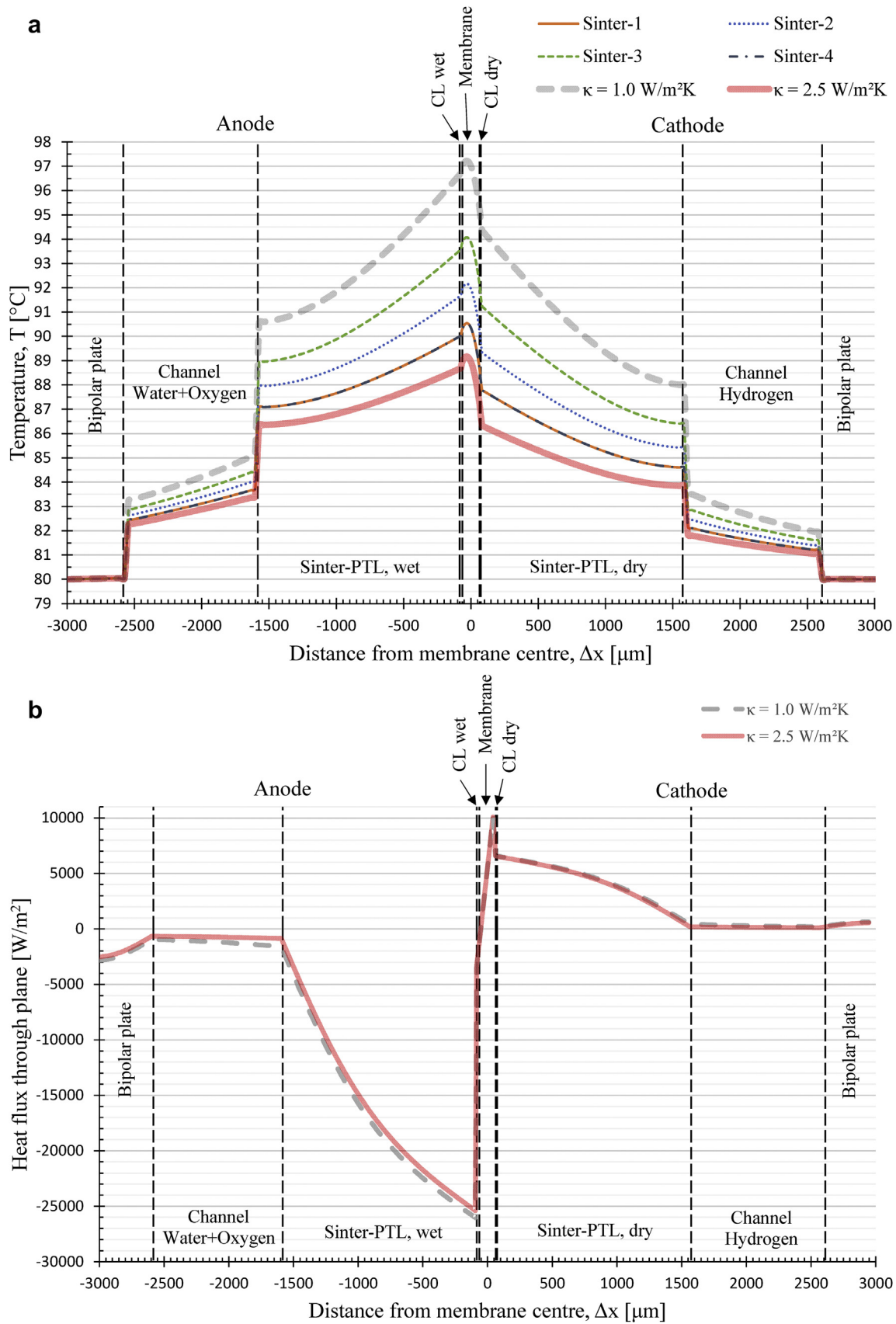
Fig. 10 – PEMWE profiles according to Case 1 (Hgas). Water on anode, hydrogen gas on cathode side. No entropic heat contribution on anode side. Dotted vertical lines represent interfaces between different materials.
