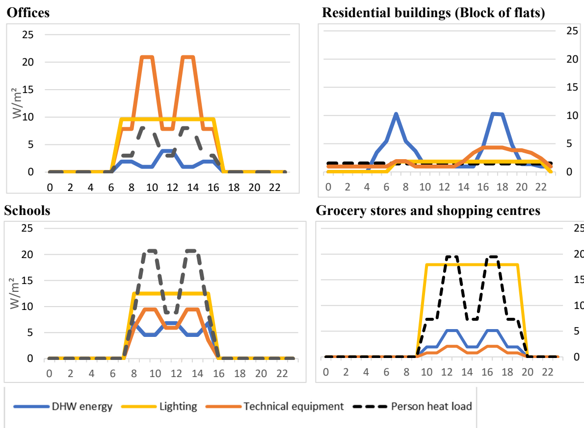
Figure 1. Load profile according to SN/TS 3031:2016.
