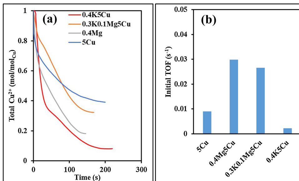
Fig. 2. (a) \text{Cu}^{2+} concentration with time on stream for the catalysts with and without promoters; (b) initial turnover frequency (TOF) of the reduction step for all the catalysts. Reaction conditions: W_{\text{cat}} = 0.3 \text{ g} , T = 230 \text{ }^\circ\text{C} , P_{\text{total}} = 1 \text{ bar} , P_{\text{C}_2\text{H}_4} = 0.1 \text{ bar} , F_{\text{tot}} = 180 \text{ ml/min} .
