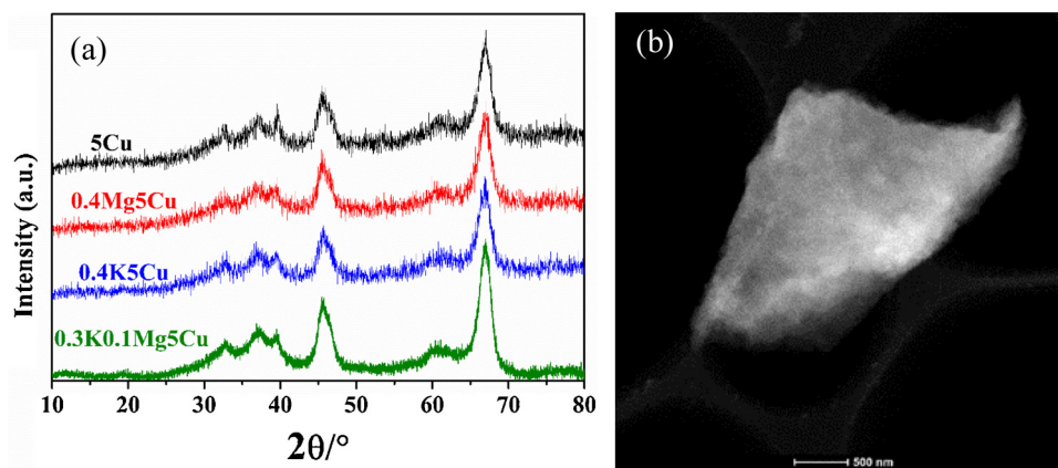
Fig. 1. (a) XRD profiles of the different catalysts; (b) TEM images of the 5Cu/Al 2 O 3 catalyst.
