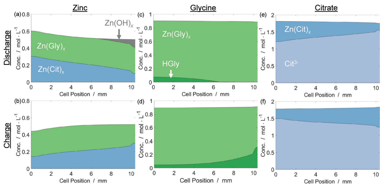
Figure 6. Anatomized concentration profiles of a,b) zinc, c,d) glycine, and e,f) citrate in the electrolyte at the end of discharging and charging. The presence of \text{Zn(OH)}_x in the discharged electrolyte but not in the charged electrolyte, combined with the increased presence of HGly in the charged electrolyte demonstrates a shift in the dominant pH buffering mechanism between discharging and charging.
