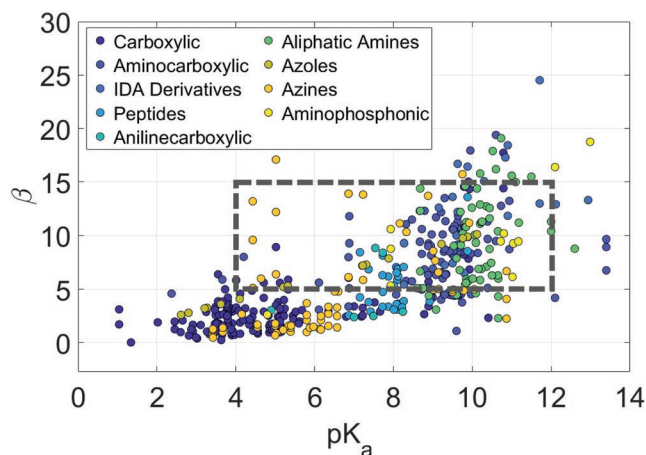
Figure 2. Zinc complex stability constant \beta = \log_{10}K_{eq} and pK a values for a selection of weak organic acids. Dashed lines indicate the approximate region of interest for aqueous pH-buffered zinc electrolyte applications. Data compiled from refs. [42–44].
