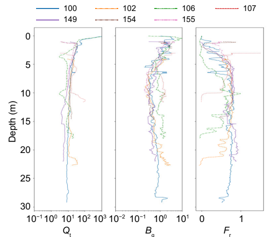
Fig. 7 Summary of CPTu at Vegvesen site in terms of the normalized parameters. References to color refer to the online version of this figure
