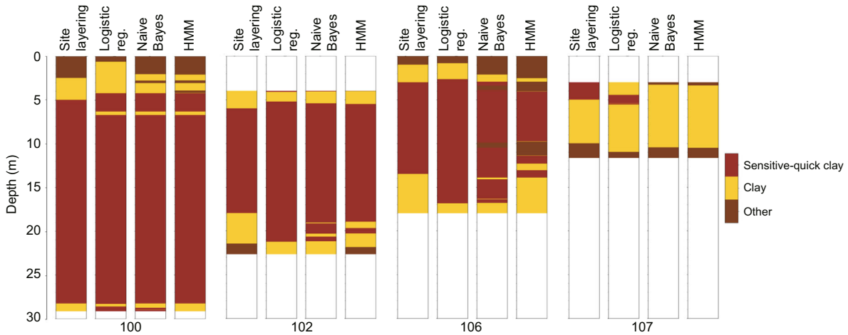
Fig. 22 Comparison of the machine learning classification for the Vegvesen dataset and the profile view of CPTus 100, 102, 106, and 107. References to color refer to the online version of this figure
