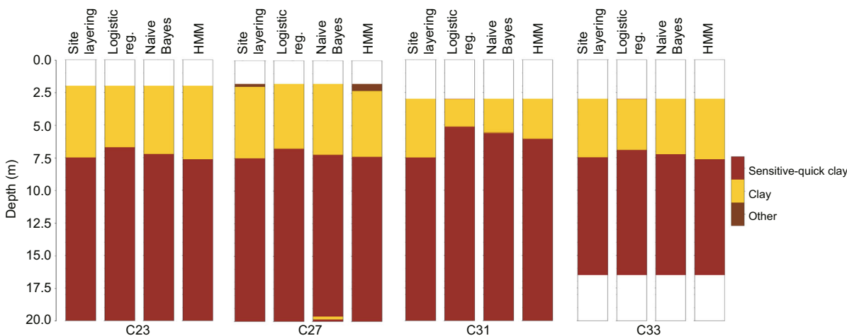
Fig. 18 Comparison of the machine learning classification for the NGTS dataset and the profile view of CPTus C23, C27, C31, and C33. References to color refer to the online version of this figure
