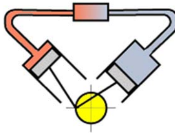
Figure 21 Principle sketch of a possible arrangement of the Stirling engine [28]
