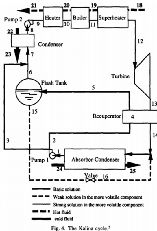
Figure 20 Principle sketch of the Kalina cycle [24]
