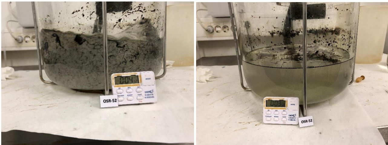
Figure 6-10 MNS test of water-free fresh ULSFO Shell 2019 at 13 °C (OSR-52). Viscosity: 33 564 mPa.s (10s -1 ). DOR 1:25. Left: Dynamic sampling. Right: Static sampling
