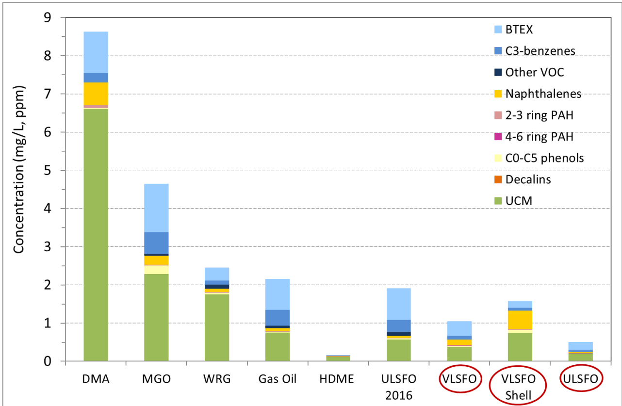
Figure 11-5 WAF concentrations of oil products tested in previous studies at SINTEF (Faksness and Altin (2017), compared with the WAFs studied here: VLSFO (Chevron), VLSFO Shell (2019), and ULSFO (Shell 2019) in red circles
