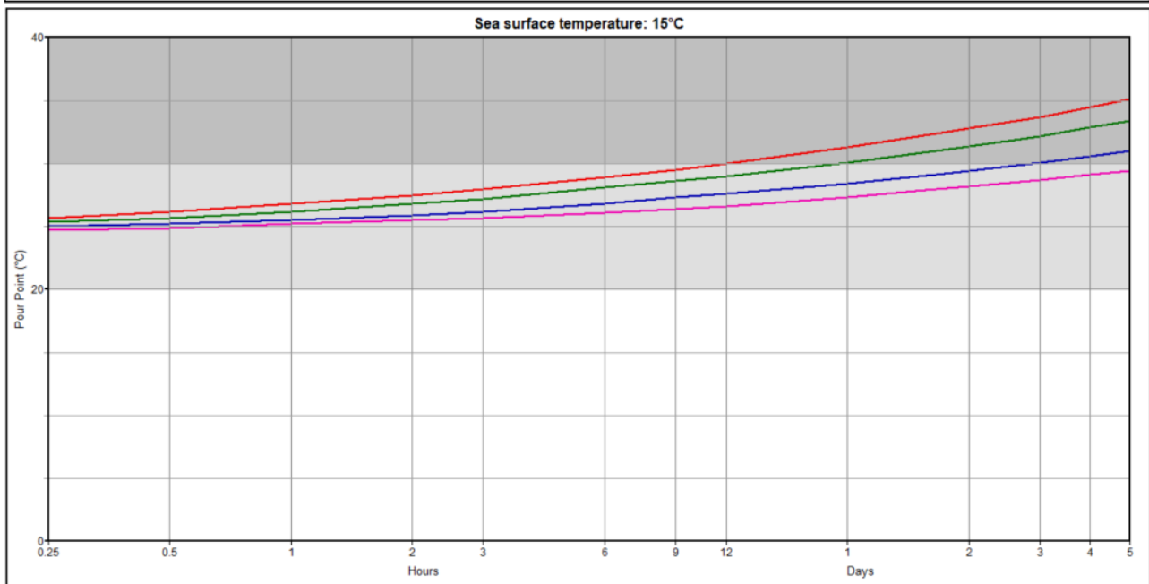
Figure C-23 Pour point ULSFO Shell 2019 at sea temperatures of 2 and 15 °C
