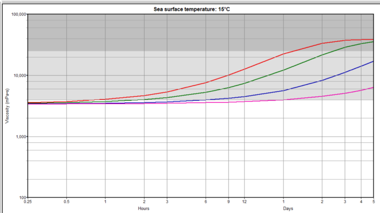
Figure C-3 Emulsion viscosity of VLSFO Chevron 2019 at sea temperatures of 2 and 15 °C
