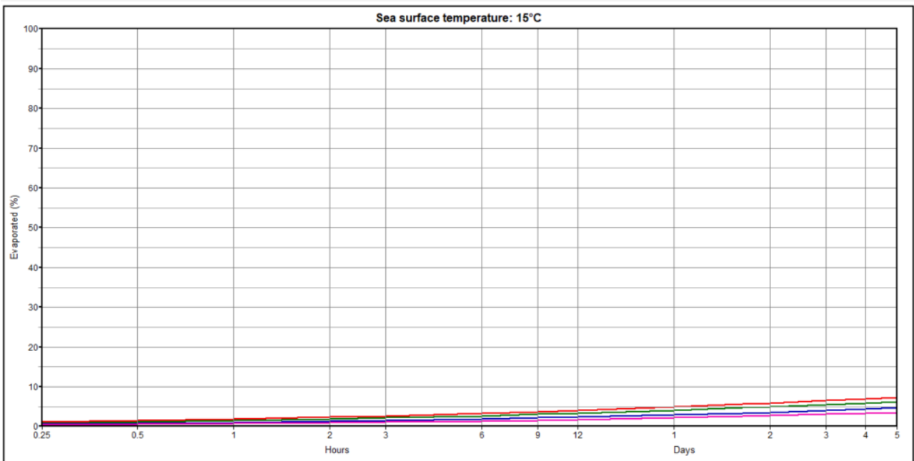
Figure C-19 Evaporative loss ULSFO Shell 2019 at sea temperatures of 2 and 15 °C
