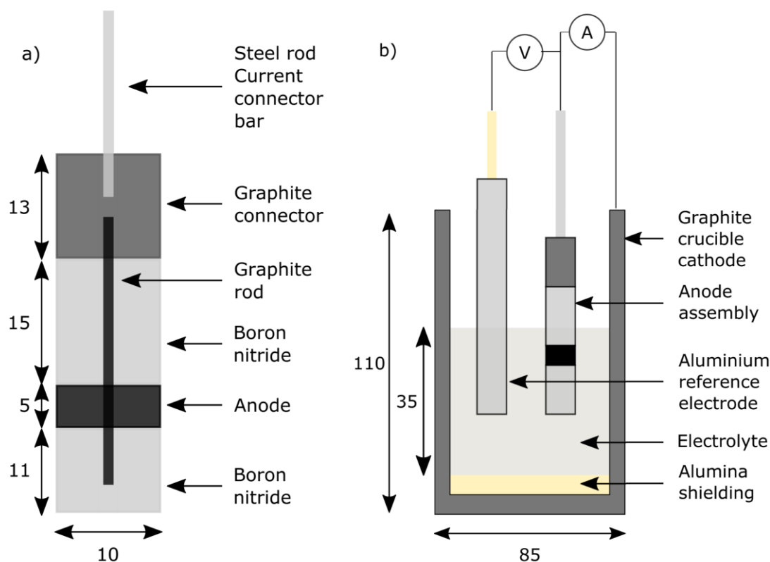
Figure 1. Electrochemical experimental setup used when electrolysing samples for CT scanning and during general electrochemical testing. All measures are in mm. a) Vertical anode assembly. b) A principle sketch of the laboratory scale electrolysis cell.
