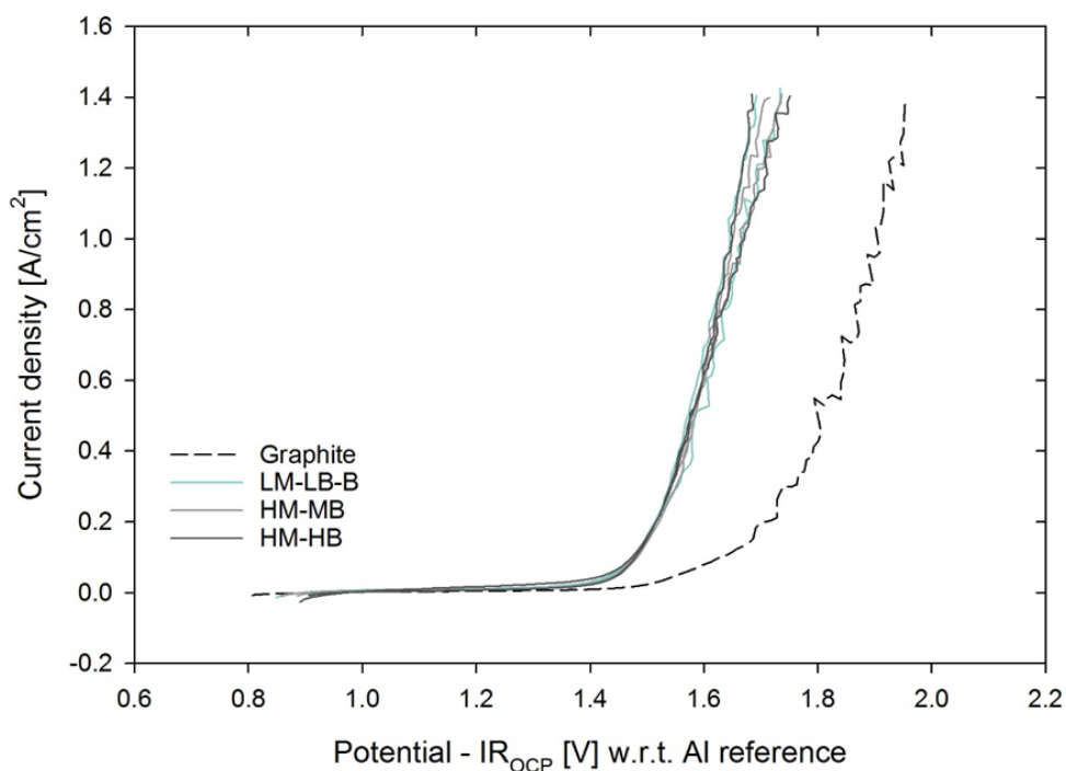
Figure 5. a) Chronopotentiometry measurements at 1.0 A/cm 2 . Graphite was used as anode reference material. b) IR corrected polarisation curves for the same anodes.
