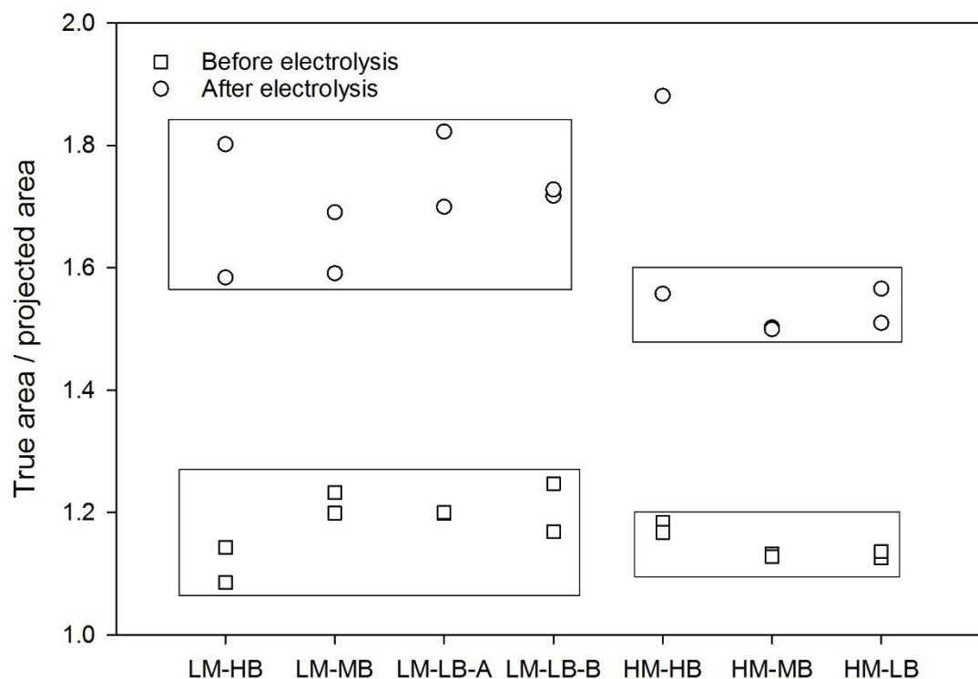
Figure 4. Ratio of true area over projected area obtained by confocal microscopy on freshly cut and ground samples and electrolysed samples (circles) at 1.0 A/cm 2 for 25 mins. The low and high mixing temperature anodes have been "boxed" together.
