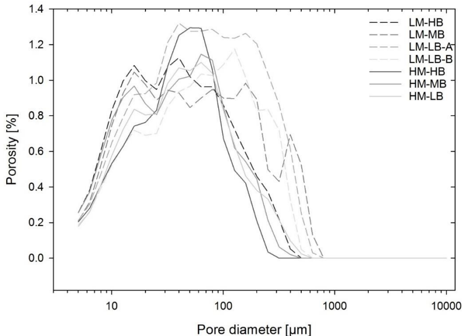
Figure 2. Porosity vs. pore diameter size obtained by optical microscopy. The results are averages between two or four parallels.
