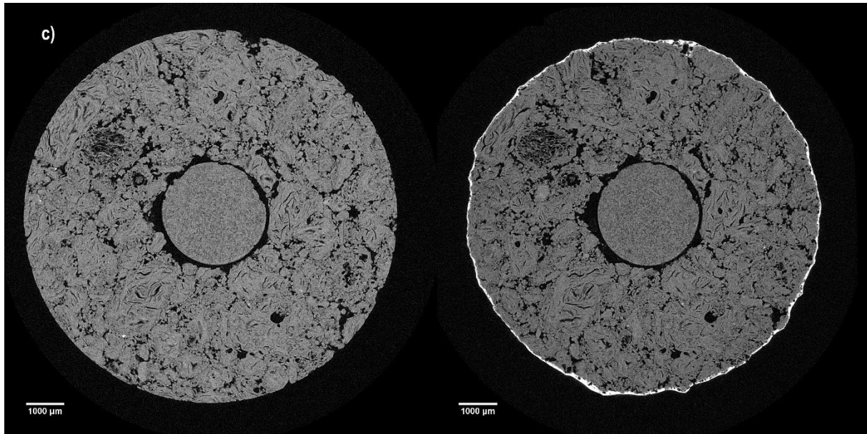
Figure 3. CT images of an interior cross-section of some selected anodes before (left) and after (right) electrolysis. a) Anode LM-LB-B, b) Anode LM-MB and c) Anode HM-HB
