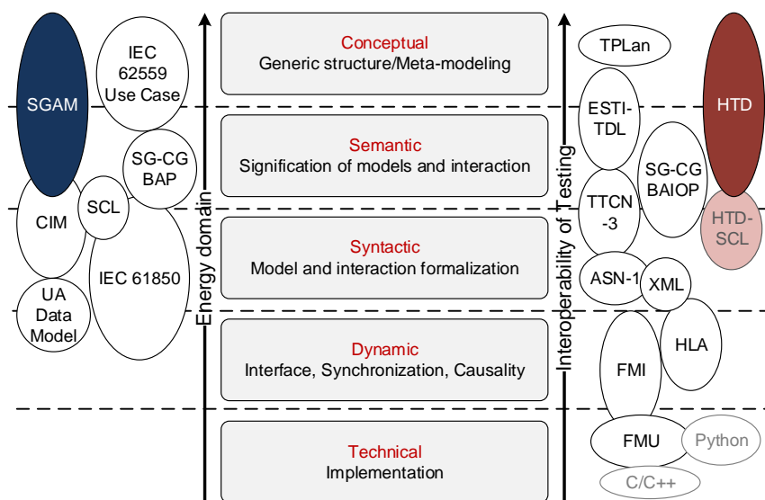
Figure 2. Abstraction layers of a holistic test and the related standards.
