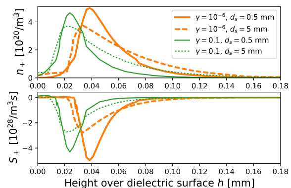
Figure 5 A higher photoemission efficiency \gamma moves the streamer closer to the dielectric surface. Positive charge species n_+ and source S_s (equation (3)) above the dielectric surface shown, d_s = 0.5 \text{ mm} and d_s = 5 \text{ mm} behind the streamer head. The source is negative since positive species are recombining in the channel. The streamer has propagated 10 \text{ mm} along the barrier surface (same as in Figure 6). Geometry G1.
