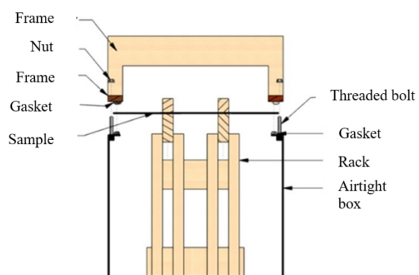
Fixing of the different samples to the airtight box.
