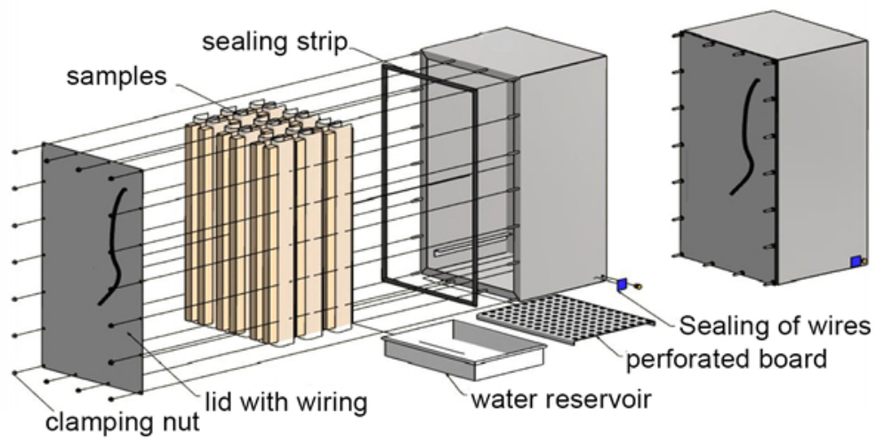
Configuration of the experimental setup.
