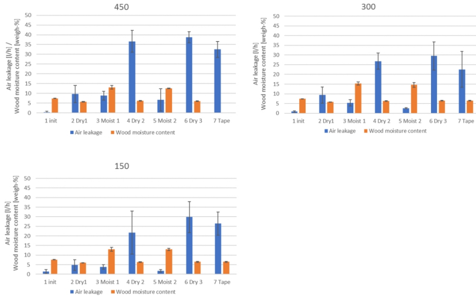
Air leakage through the different samples before and after drying and moistening. The code e.g. " 450" means the centre to centre distance of the fasteners in mm.
