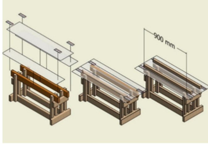
Mounting of the test samples.
