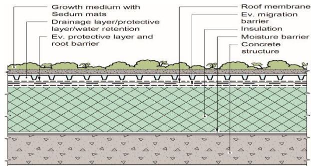
Figure 1: Composition of a green roof assembly on a compact, flat roof (Skjeldrum and Kvande, 2017).
